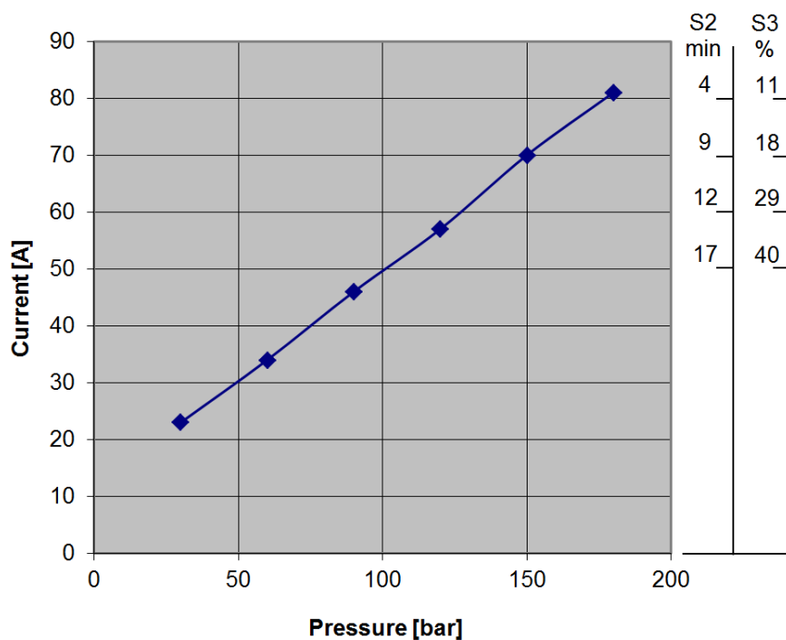
Electrical curve
