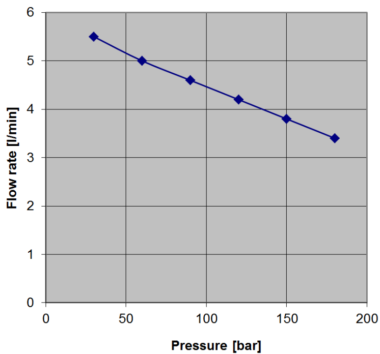
Hydraulic curve
