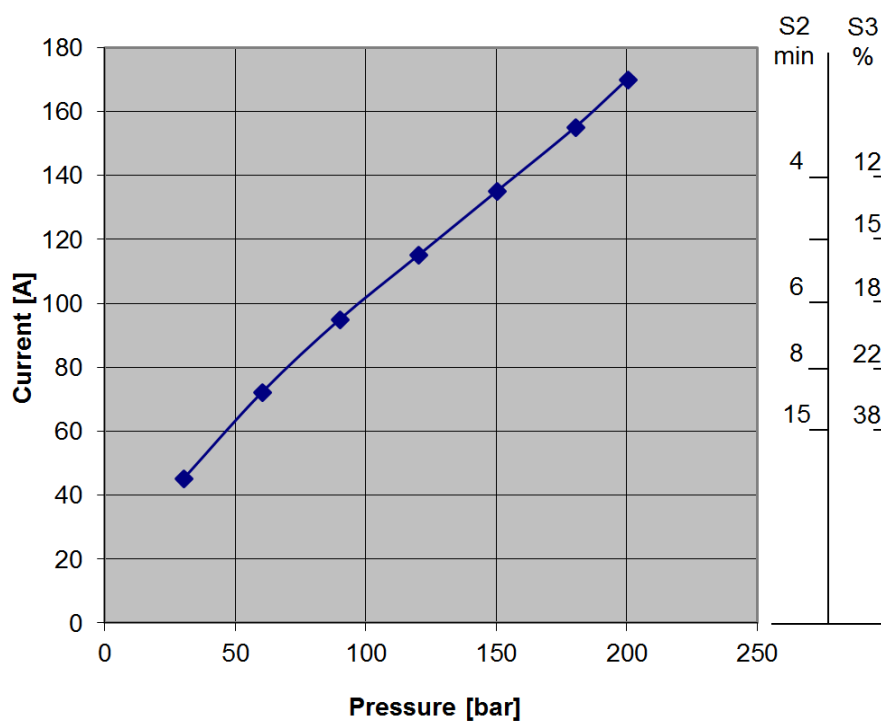
Electrical curve
