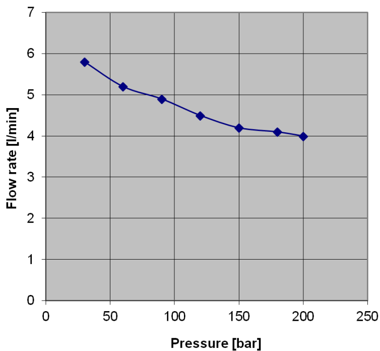
Hydraulic curve
